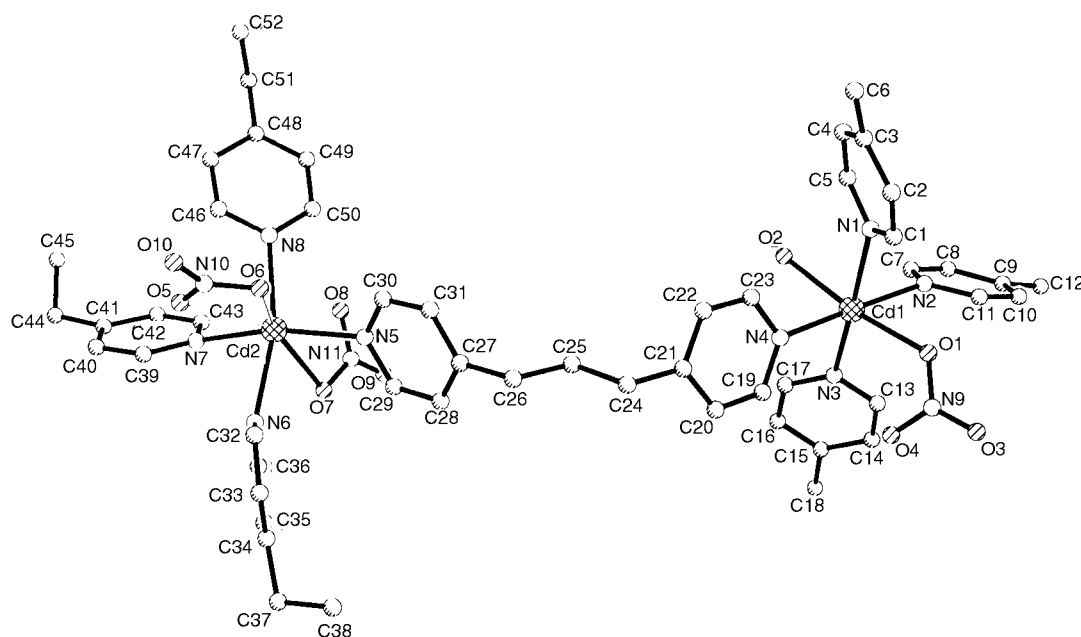
Fig. 3 Building block of structure 2 showing the atom numbering scheme.
