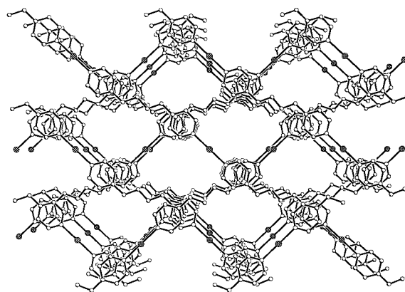
Fig. 11 Criss-cross arrangement of adjacent chains in 4 , view along [001]. The chains run along [110] and [1\bar{1}0] ( \text{H}_2\text{O} and \text{NO}_3 omitted for clarity).
