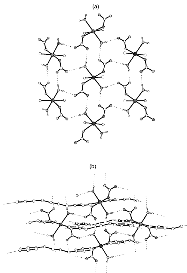
Fig. 12 (a) Two-dimensional hydrogen network in 4 , view along [100] (C and H atoms omitted for clarity). O4–H1O \cdots O3c [2.13(3), 2.994(3) Å; 171(3) ^\circ ]; O4–H2O \cdots O2d [2.11(4), 2.904(3) Å; 164(3) ^\circ ]; symmetry operations: a: x, -y + 1/2, z + 1/2 ; x, y, z + 1 . (b) Connection of the infinite chains via hydrogen bonds.
