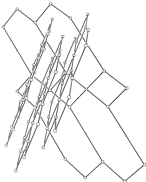
Fig. 9 Schematic representation of the 3-D inclined interpenetration of nets in 3 . The positions of Cd2 (small circles) are not nodes of the network. The SO 4 rods connecting adjacent sheets are omitted for clarity.
